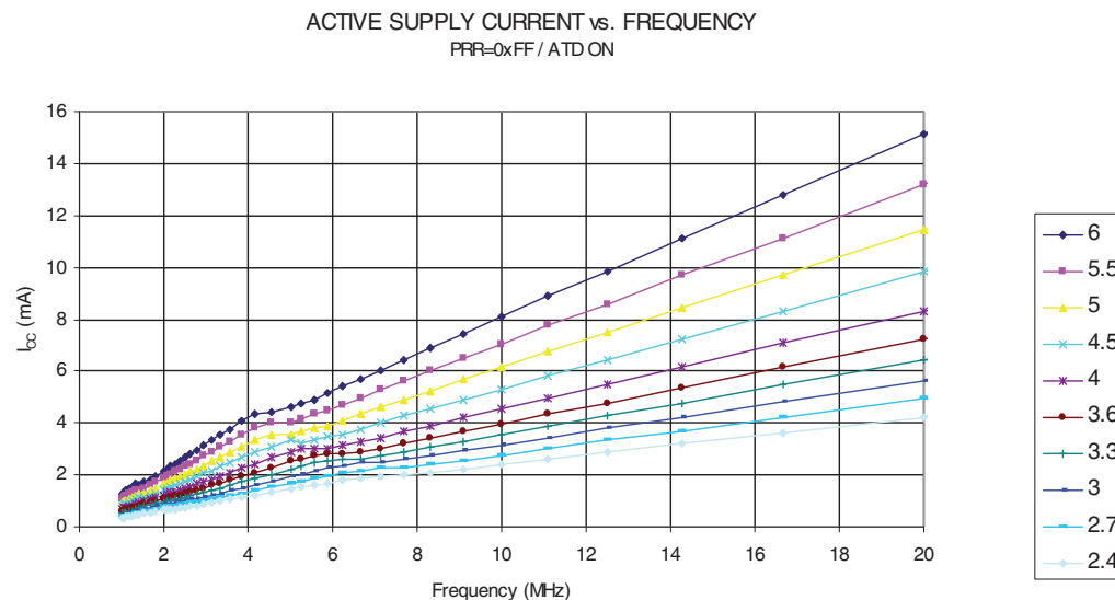
Figure 4-116. Active Supply Current versus Frequency ( \geq 1\text{MHz} )
